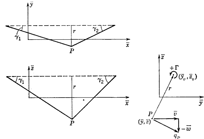
FIG. 6-8. Vortex line segment of Biot-Savart law.
