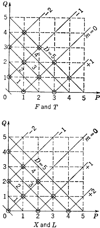
FIG. 10-31. PQ diagram for missile with 2-gonal and mirror symmetries.
