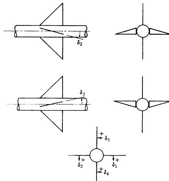
FIG. 8-2. Positive deflection angles. Top left, side view; center left, top view; bottom, end view.
