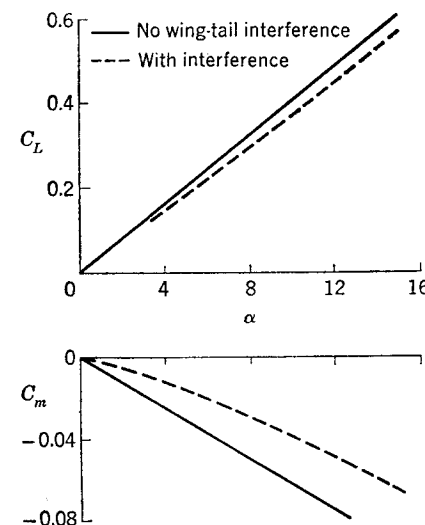
FIG. 7-10. Calculated lift and moment curves of example configuration.
