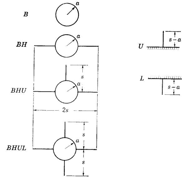
FIG. 10-27. Components in build-up of cruciform empennage.
