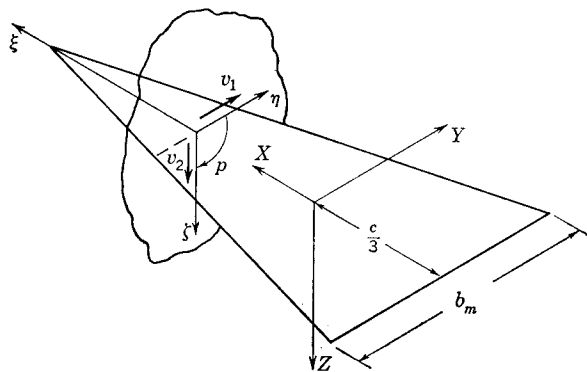
FIG. 10-8. Axes and notation for slender triangular wing.
