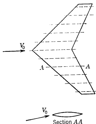
Fig. 2-2. Strip theory.
