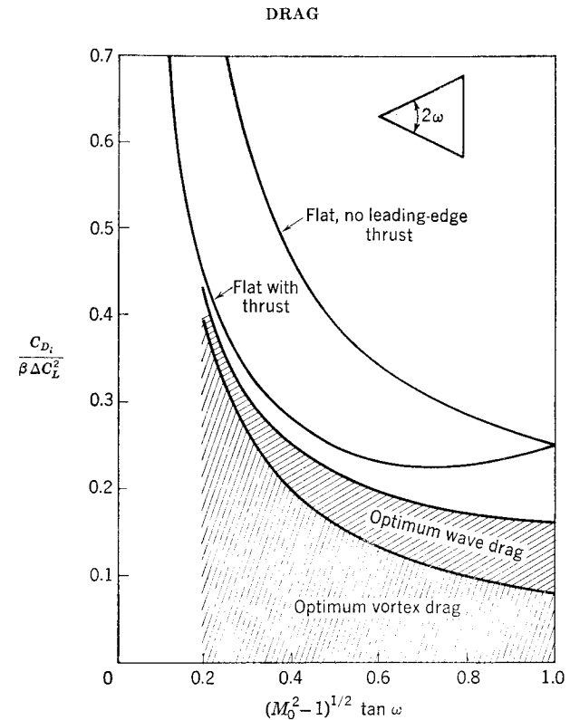
FIG. 9-23. Drag due to lift for triangular lifting surfaces.
