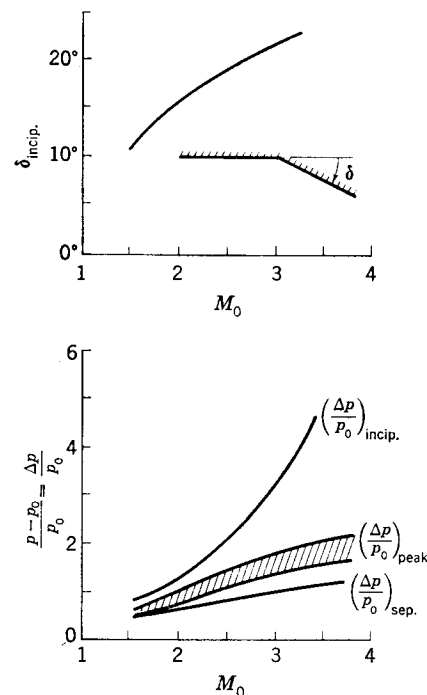
FIG. 8-27. Control deflection and pressure ratio for incipient separation of supersonic turbulent boundary layer.
