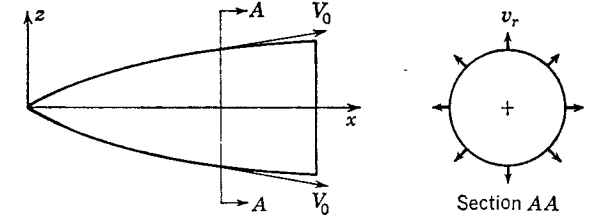
FIG. 3-2. Source flow in crossflow plane of body of revolution.
