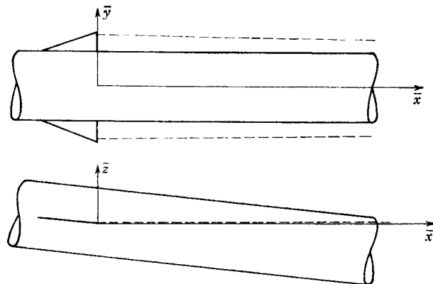
FIG. 6-18. Paths of vortices behind panel of wing-body combination; a/s_m = 0.6 .
