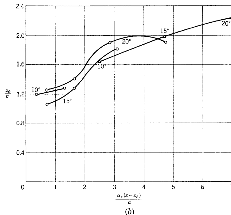
FIG. 4-17. Vortex positions for bodies of revolution. (a) Lateral location; (b) vertical location.
