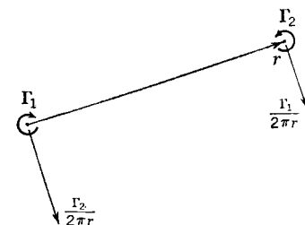
FIG. 6-5. Mutual induction between pair of two-dimensional vortices.
