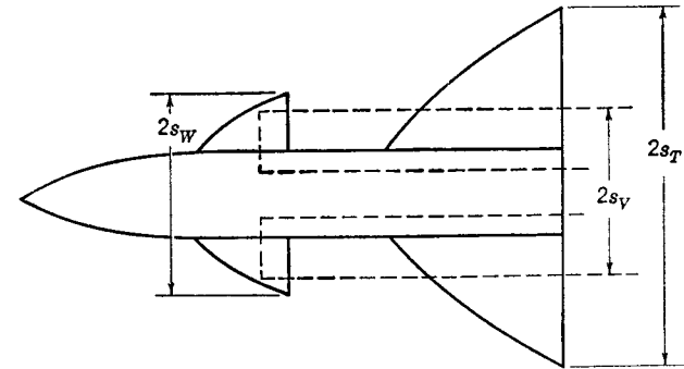
FIG. 7-7. Model of wing vortices impinging on tail.
