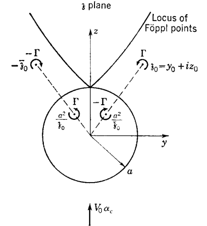
FIG. 4-19. Symmetrical vortex pair in presence of circular cylinder.
