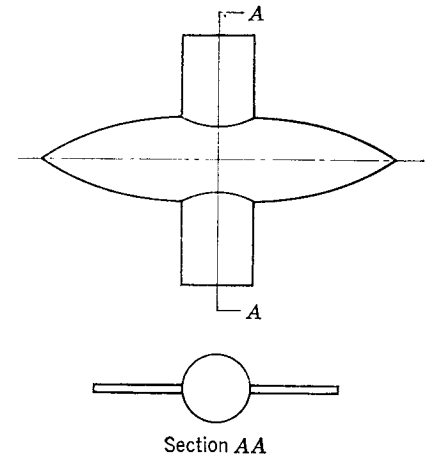
FIG. 9-18. Indentation of body to minimize pressure drag at zero angle of attack according to NACA area rule.
