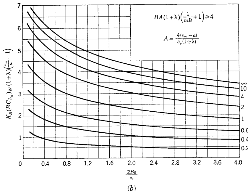
FIG. 5-13. Values of K_B based on planar model. (a) No afterbody; (b) afterbody
