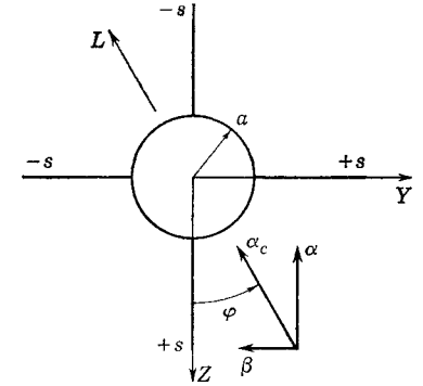
FIG. 10-15. Crossflow plane at wing trailing edges of slender cruciform missile.
