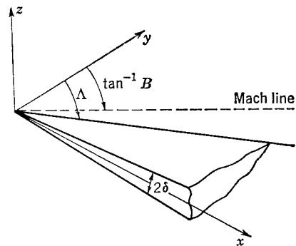
FIG. 2-3. Infinite wedge or infinite triangular cone.
