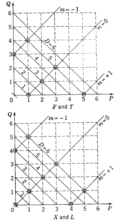
FIG. 10-28. PQ diagrams for cruciform missile.
