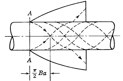
FIG. 5-11. Transference of lift from wing to body.
