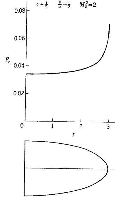
FIG. 4-7. Thickness pressure distribution for elliptical cone.
