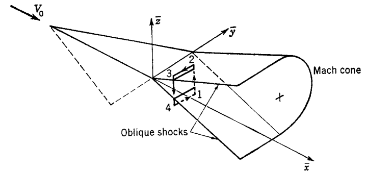
FIG. 6-3. Circulation contour with trailing shock waves.
