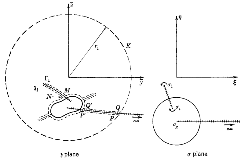
FIG. 4-23. Cuts and contours of integration.
