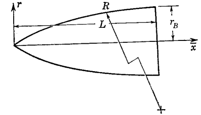
FIG. 4-2. Coordinates of tangent ogive.
