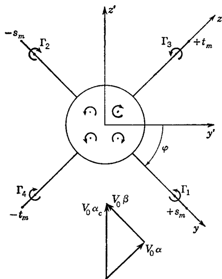
FIG. 6-24. Vortex model of cruciform wing-body arrangement.
