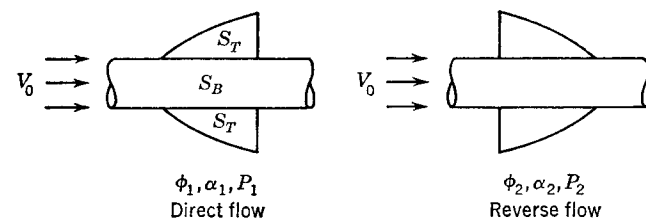
FIG. 7-12. Configuration in direct and reverse flow.
