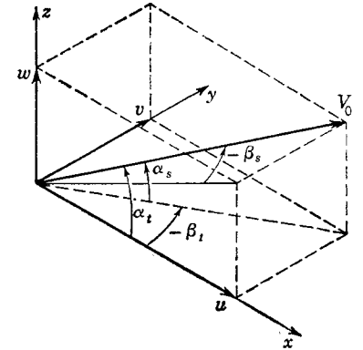
FIG. 1-3. Angles of attack and sideslip.
