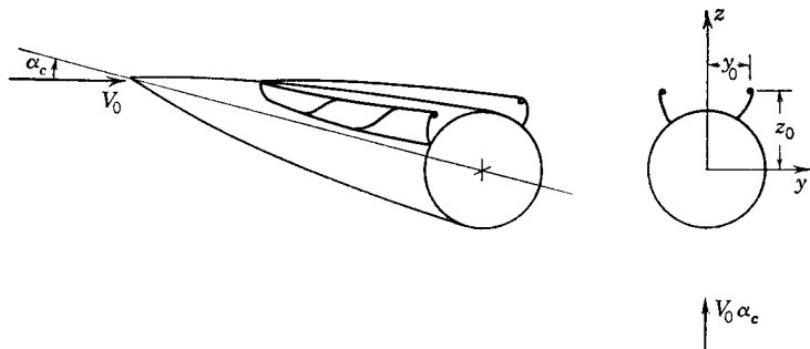
FIG. 4-14. Crossflow vortices of body of revolution.
