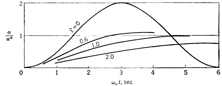
FIG. 8-30. Change in attitude of missile due to sudden application of pitch control.
