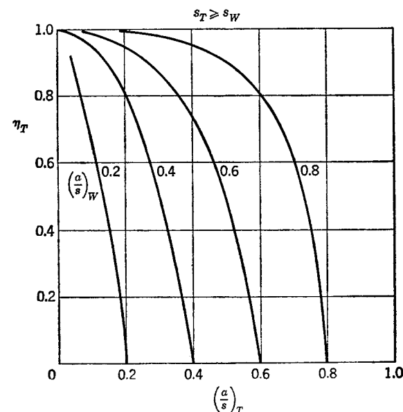
FIG. 7-2. Tail effectiveness for flat vortex sheet.
