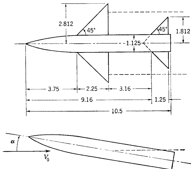
FIG. 7-9. Wing-body-tail combination of illustrative example.
