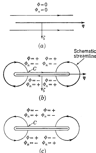
FIG. 10-9. Signs of potentials and their normal derivatives for various unit velocities. (a) Unit velocity along \eta , \phi_1 ; (b) unit velocity along \zeta , \phi_2 ; (c) unit rolling velocity, \phi_3 .
