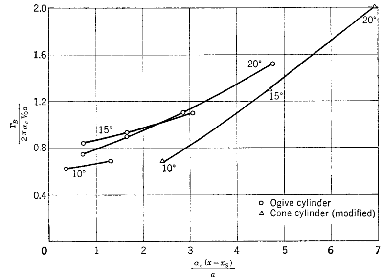
FIG. 4-16. Nondimensional vortex strengths for bodies of revolution.
