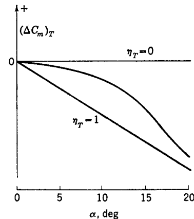
FIG. 7-16. Tail pitching-moment contribution with shock-expansion interference.
