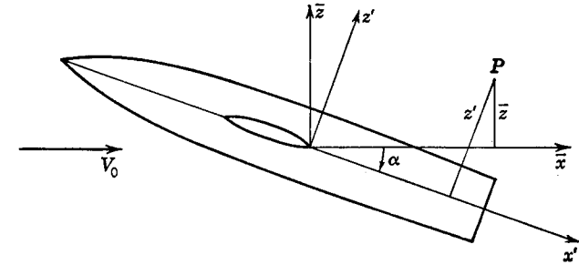
FIG. 6-15. Wind and body axes.
