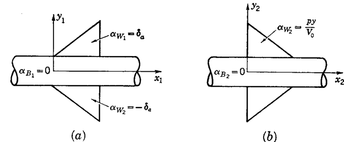
FIG. 8-8. Direct and reverse flows for calculating rolling effectiveness of planar configurations. (a) Case 1; (b) case 2.
