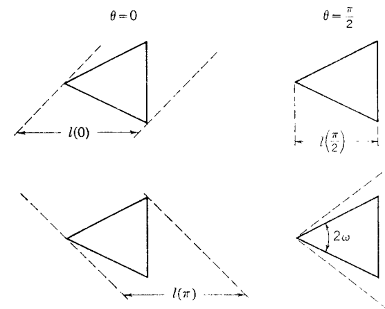
FIG. 9-24. Values of l(\theta) for triangular wings.
