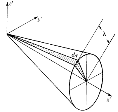
FIG. 4-8. Notation for elliptical cone.
