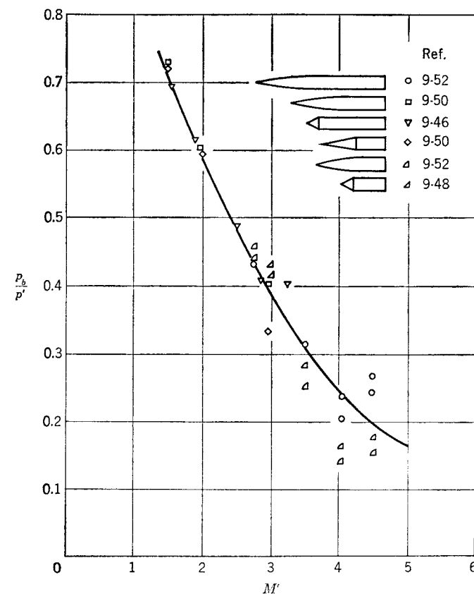
FIG. 9-30. Base-pressure correlation for bodies of revolution with relatively thin turbulent boundary layers.
