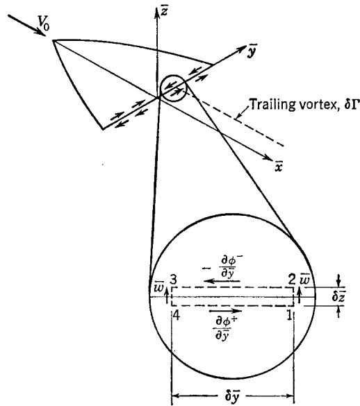
FIG. 6-1. Wind axes and sidewash at the trailing edge of the wing.
