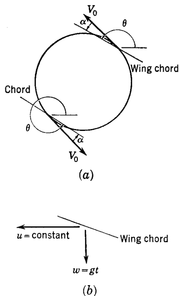
FIG. 10-19. Types of uniform motion involved in damping in pitch. (a) \alpha = 0 , q = \text{constant} ; (b) q = 0 , \dot{\alpha} = \text{constant} .
