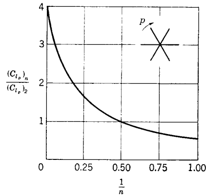
FIG. 10-14. Effect of number of fins on damping in roll.
