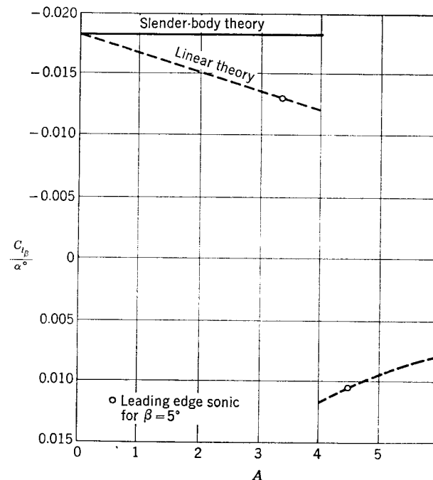
FIG. 10-22. Rolling moment due to sideslip of triangular wings; M_0 = 2 .
