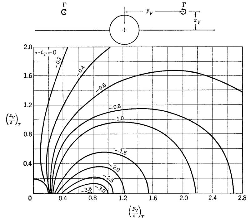
FIG. 7-8. Chart of tail interference factor based on strip theory; \lambda_T = 0 , (a/s)_T = 0.2 .
