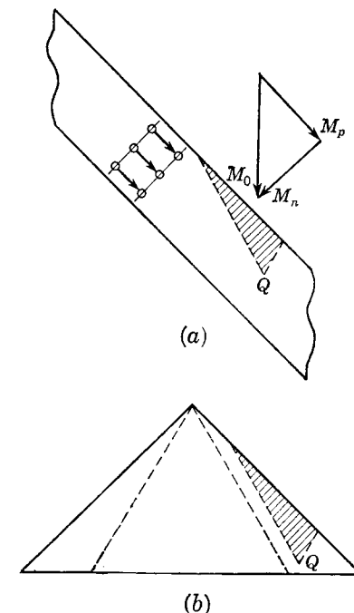
FIG. 2-10. Simple sweep theory with application to triangular wing with supersonic leading edges. (a) Infinite swept wing; (b) triangular wing.
