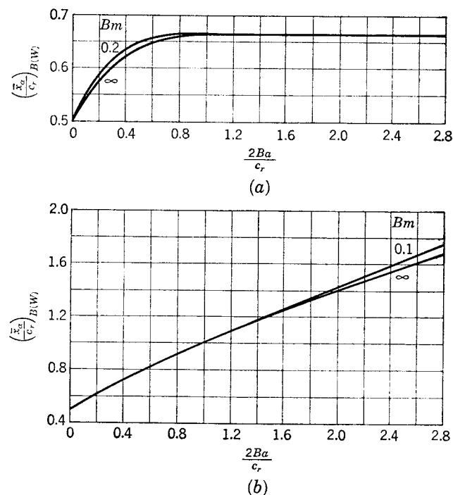
FIG. 5-14. Values of (\bar{x}_a/c_r)_{B(W)} based on planar model. (a) No afterbody; (b) afterbody.
