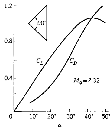
FIG. 8-28. Maximum lift characteristics of triangular wing at supersonic speed.
