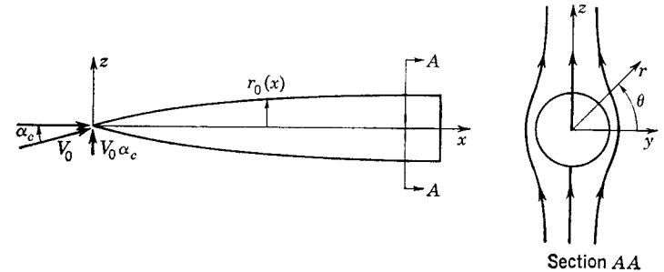
FIG. 3-3. Incompressible crossflow around body of revolution at angle of attack.
