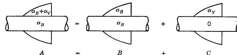
FIG. 7-13. Decomposition of twisted tail configuration into components.
