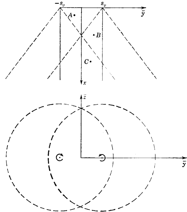
FIG. 6-10. Regions of influence of supersonic horseshoe vortex.
