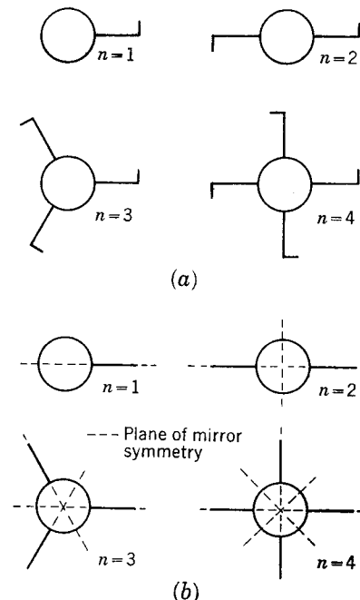
FIG. 10-3. Examples of missile symmetries. (a) N -gonal symmetry, no mirror symmetry; (b) N -gonal and mirror symmetries.
