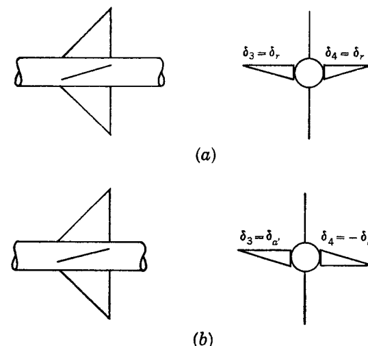
FIG. 8-4. (a) Yaw control and (b) roll control with vertical controls.
