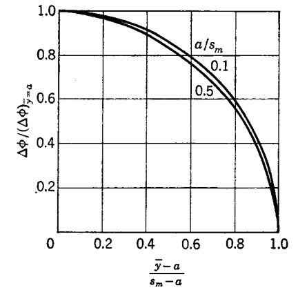
FIG. 6-12. Potential-difference distribution at trailing edge of wing in combination with body according to slender-body theory.
